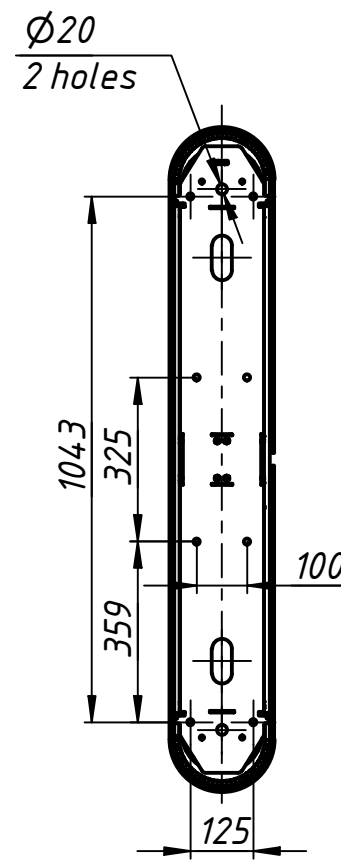
Instalation tamplate
